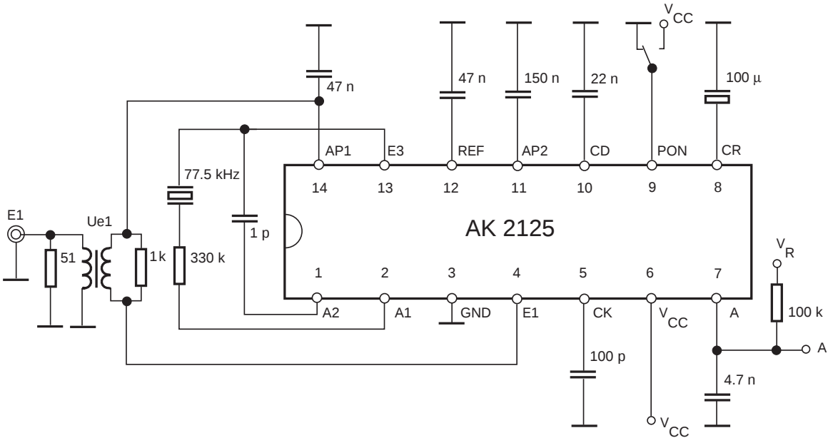
Ue1 : pot core A_L 1100 \text{ nH/w}^2 ; 2 x 25 windings with 0.2 CuL
