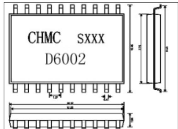
Outline Drawing
